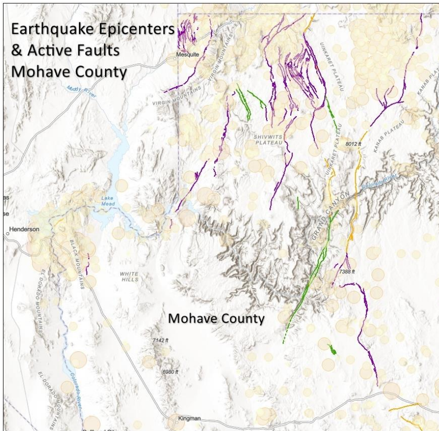
Figure x. Earthquake epicenters (light orange circles) and Quaternary faults of Mohave County (purple, gold and green lines or line segments). Epicenter circle size increases with increasing earthquake magnitude. Hundreds of earthquakes have occurred in Mohave County and environs.
