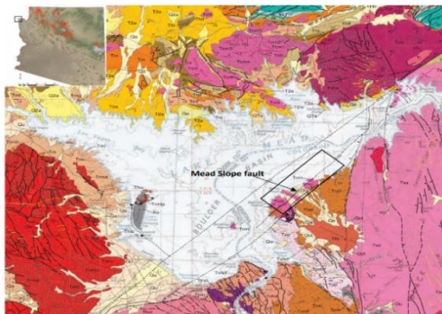
Mead Slope Fault Zones
