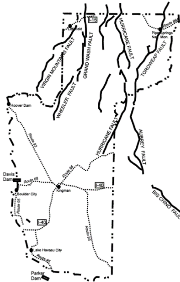
Mohave County Fault Zone Map
