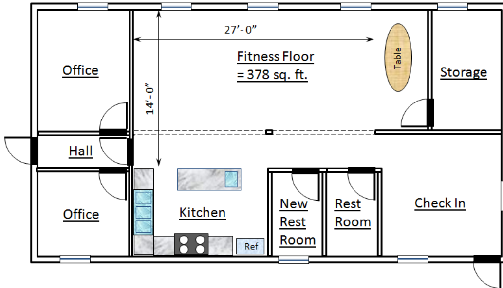
Conceptual Floor Plan
